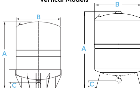
Vertical Models
